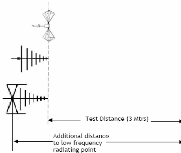
Figure 5 - Definition of antenna to EUT distance
