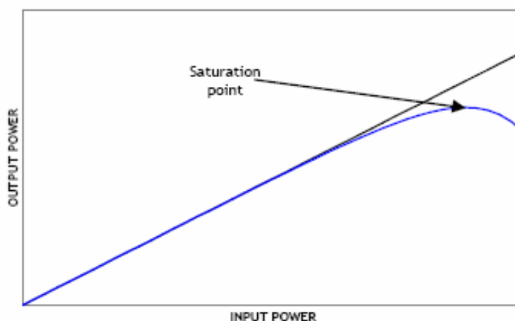
Figure 1 - Amplifier gain curve
