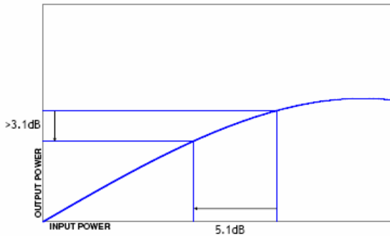
Figure 4 -2dB Linearity Criteria
