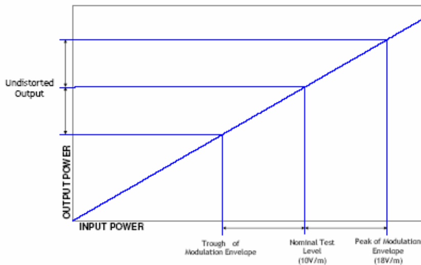
Figure 3 - Amplifier operated in linear range
