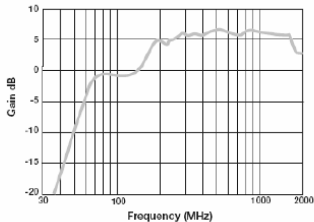
Figure 6 - Antenna gain vs. frequency
